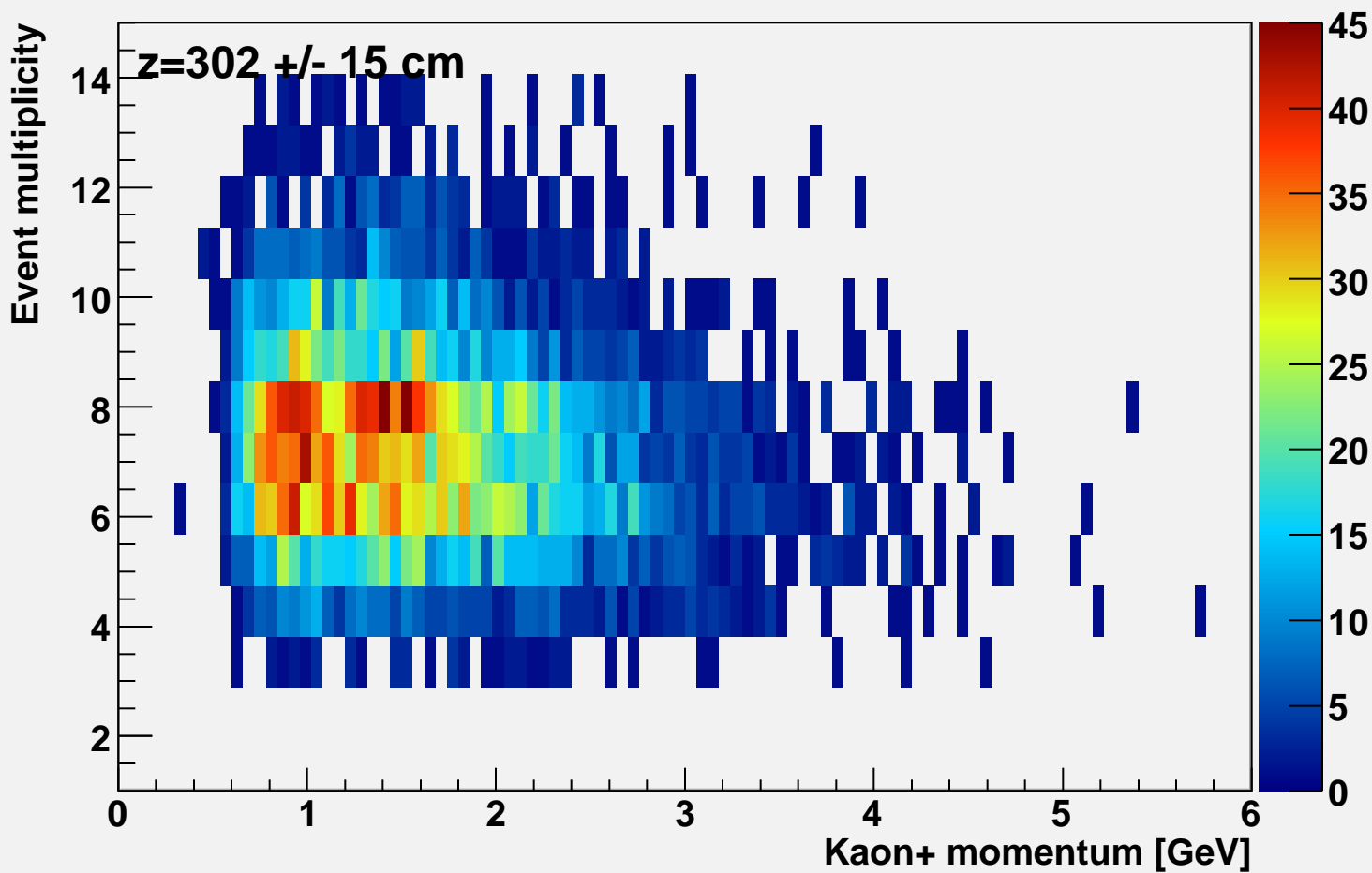
Event multiplicity vs k-momentum at bcal z=302
