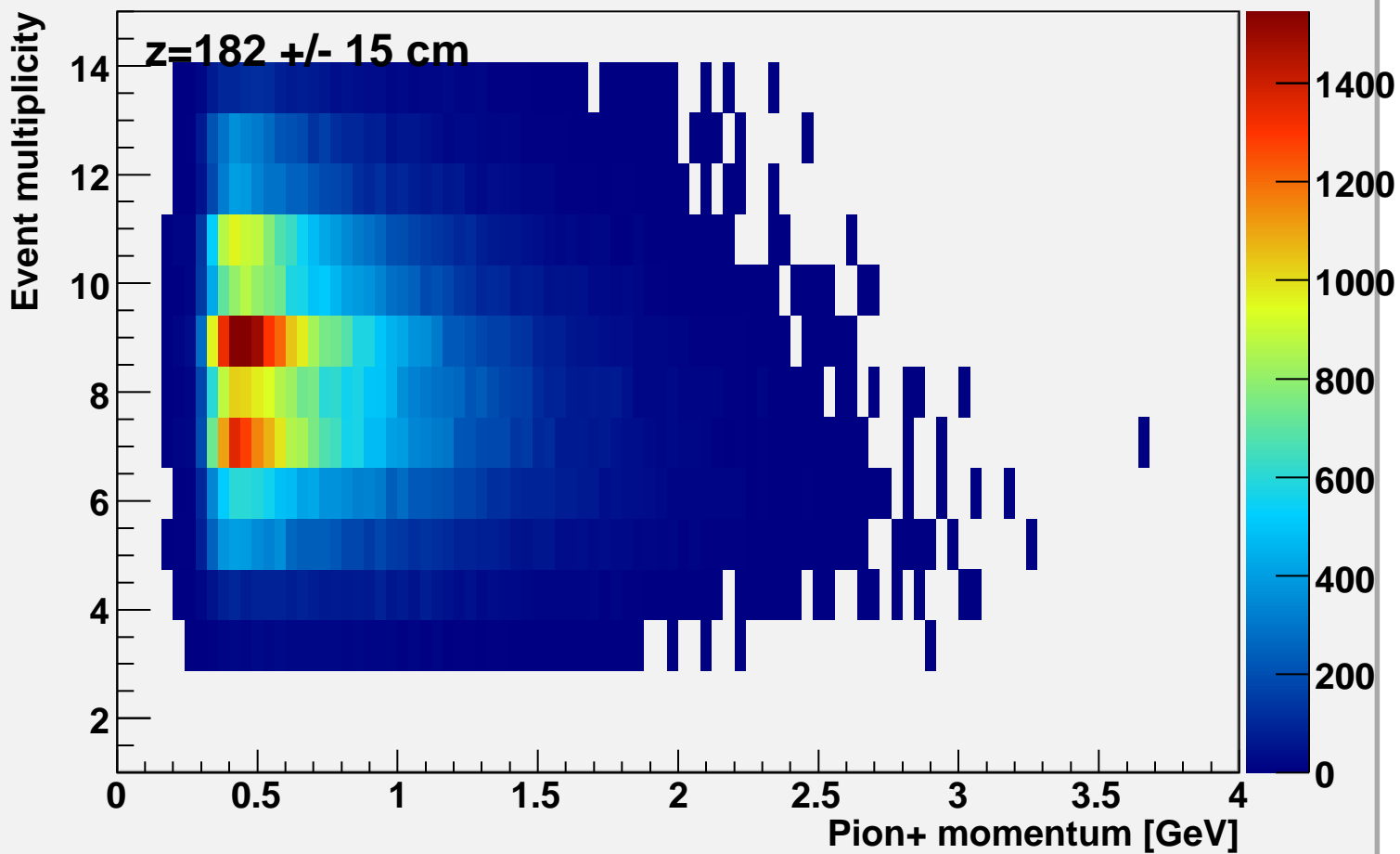
Event multiplicity vs pi-momentum at bcal z=182
