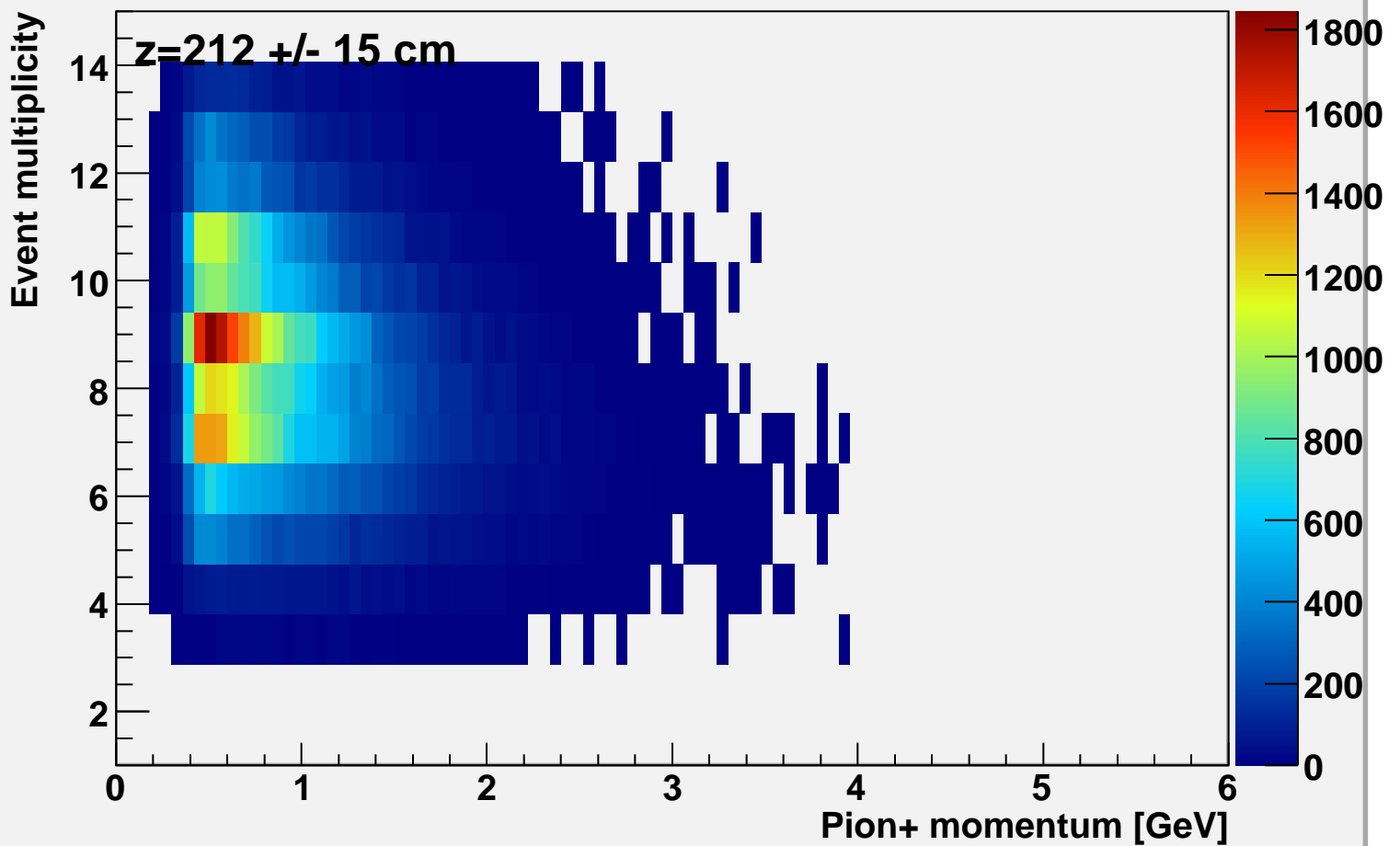
Event multiplicity vs pi-momentum at bcal z=212
