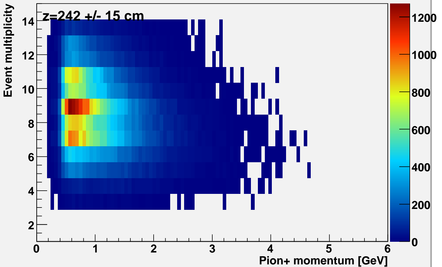
Event multiplicity vs pi-momentum at bcal z=242
