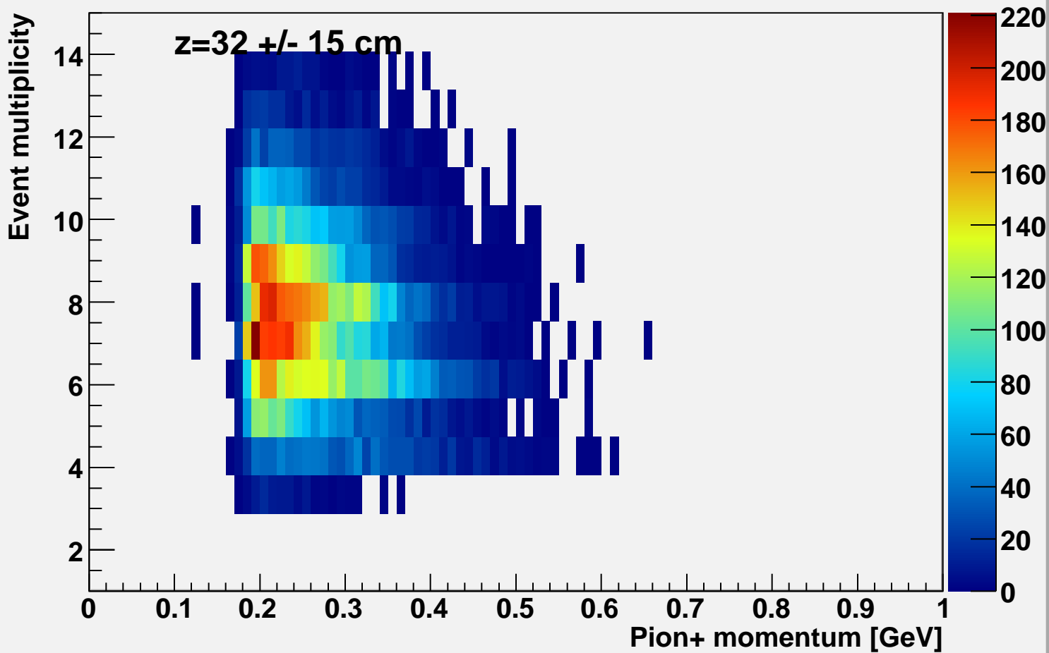
Event multiplicity vs pi-momentum at bcal z=32
