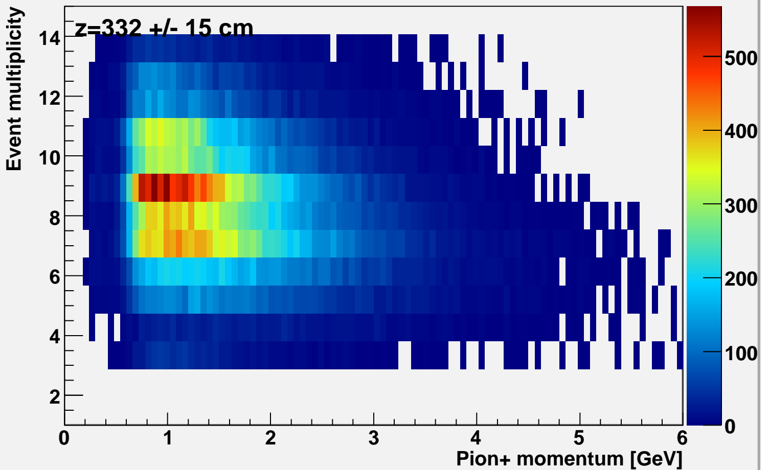
Event multiplicity vs pi-momentum at bcal z=332
