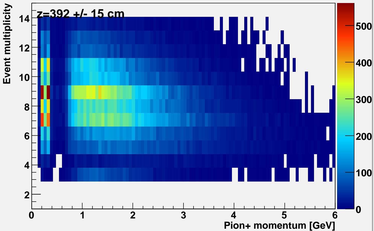
Event multiplicity vs pi-momentum at bcal z=392
