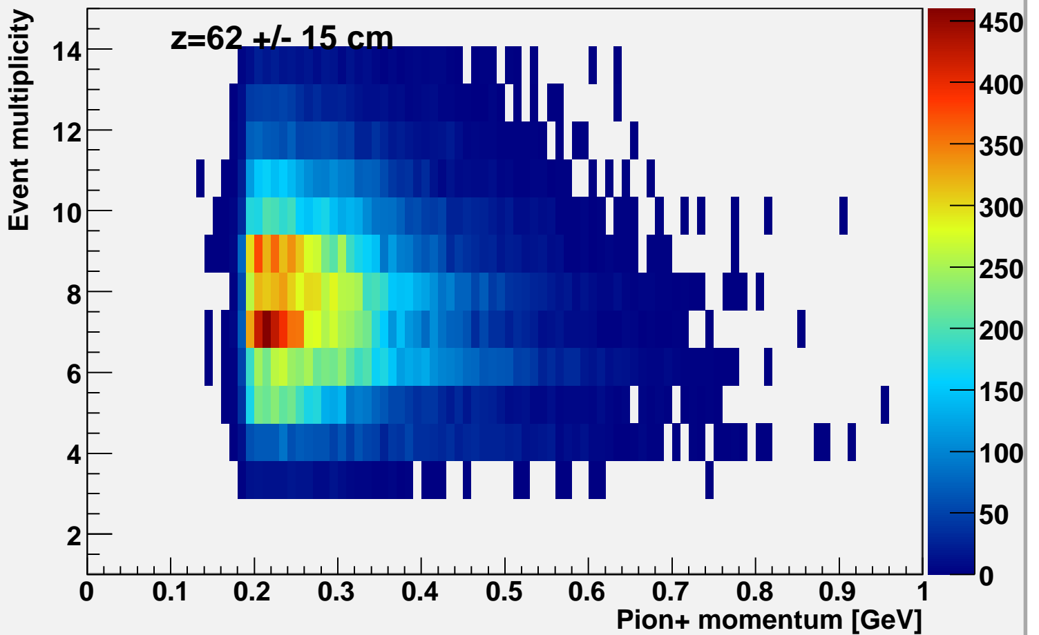
Event multiplicity vs pi-momentum at bcal z=62
