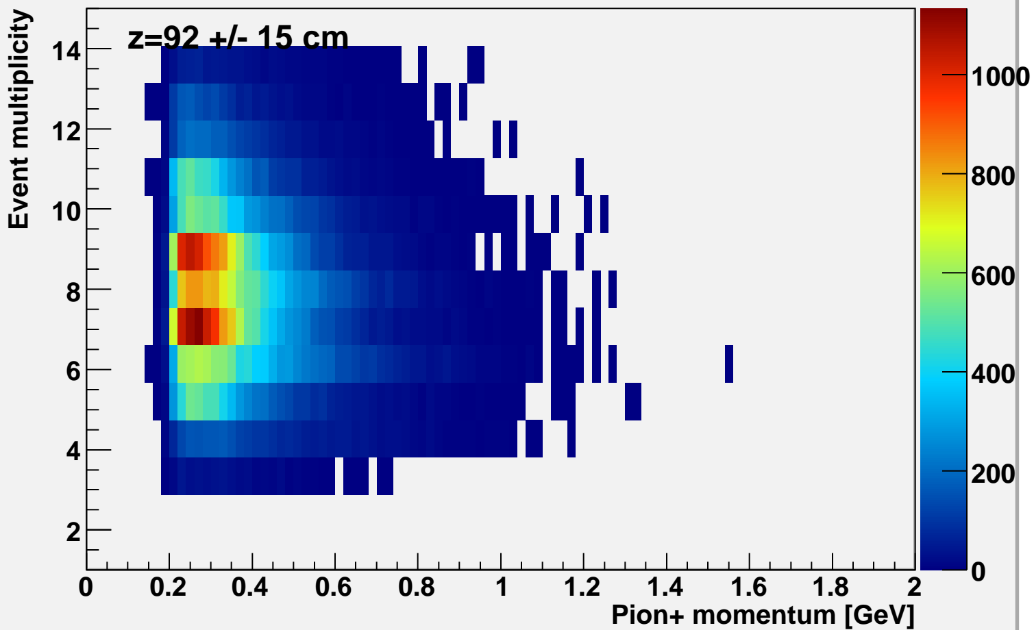
Event multiplicity vs pi-momentum at bcal z=92
