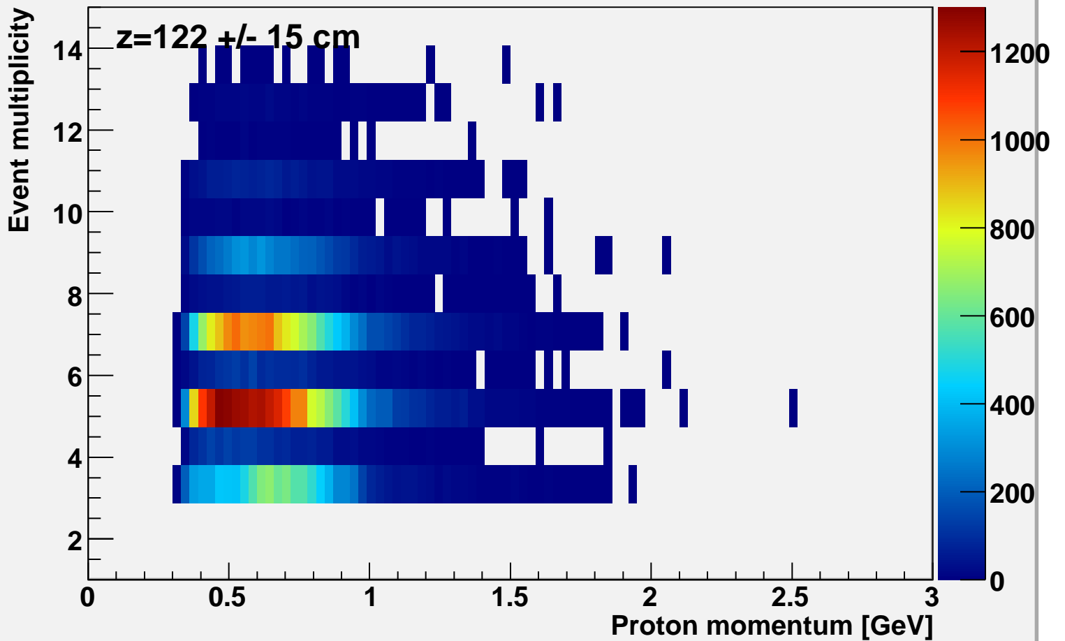
Event multiplicity vs p-momentum at bcal z=122
