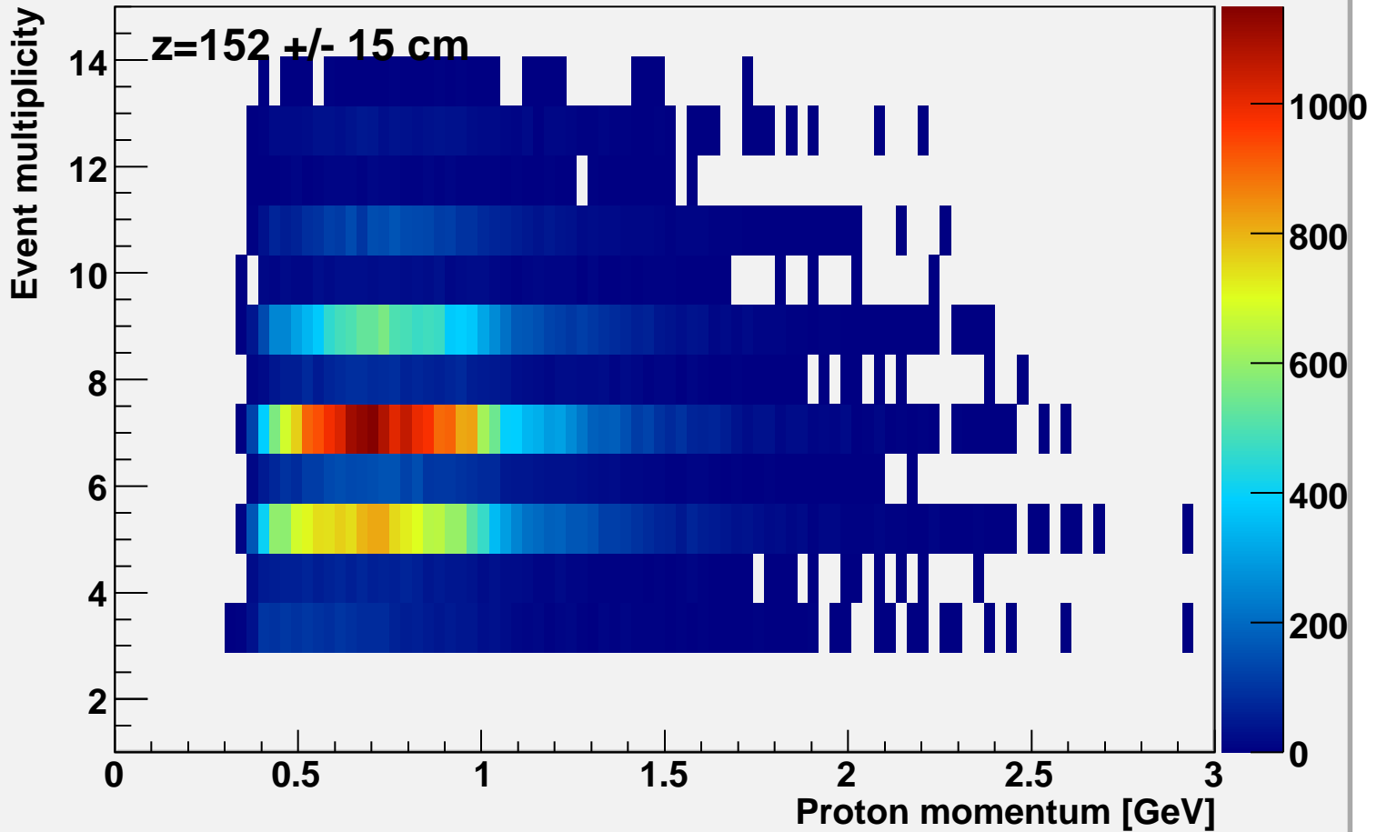
Event multiplicity vs p-momentum at bcal z=152
