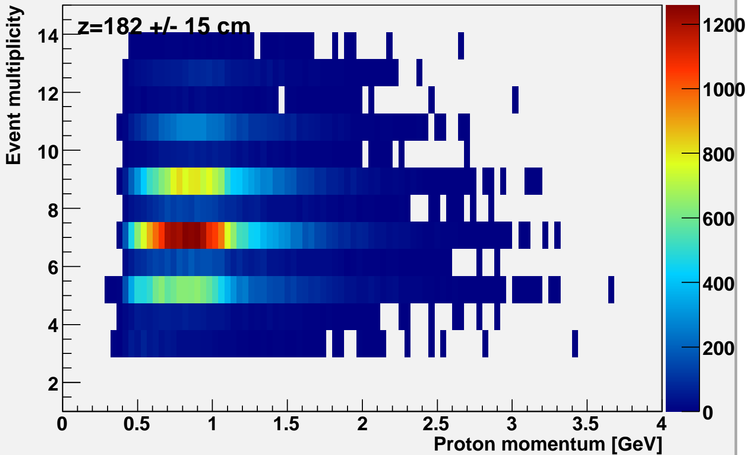
Event multiplicity vs p-momentum at bcal z=182
