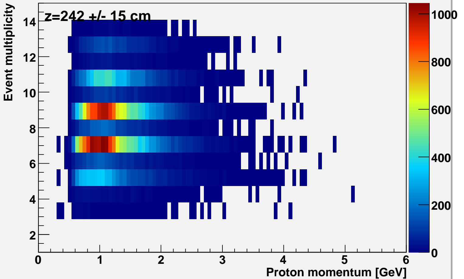
Event multiplicity vs p-momentum at bcal z=242
