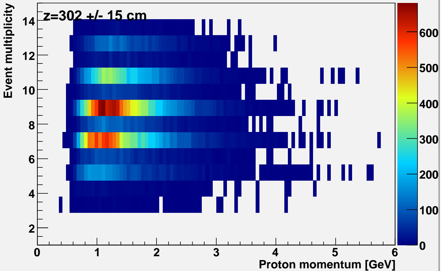
Event multiplicity vs p-momentum at bcal z=302
