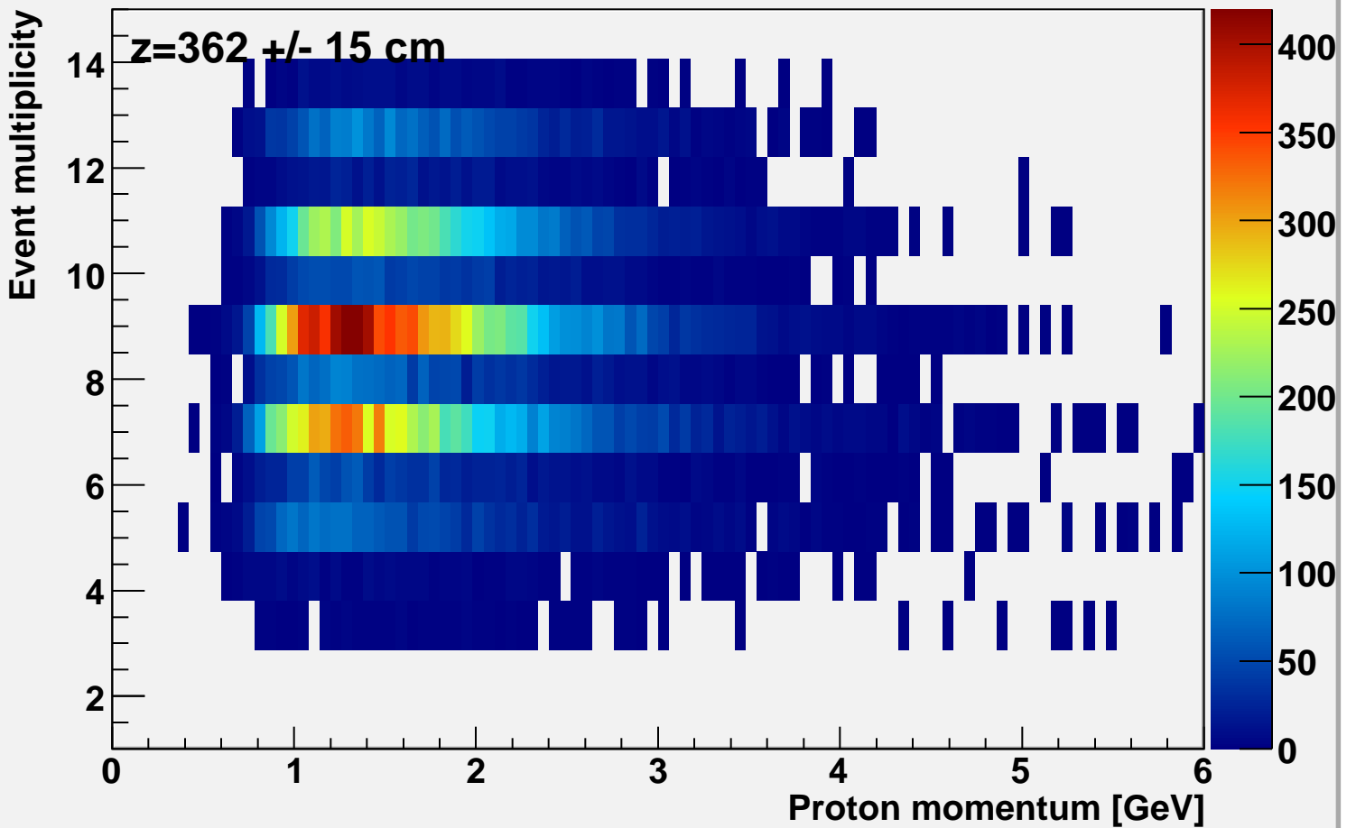
Event multiplicity vs p-momentum at bcal z=362
