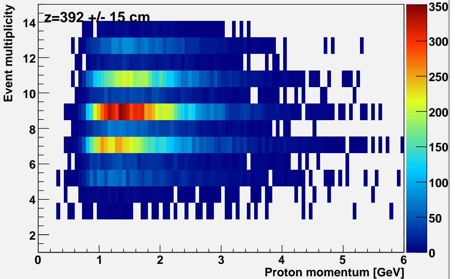
Event multiplicity vs p-momentum at bcal z=392
