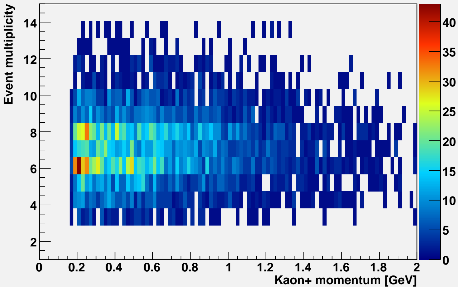
Event multiplicity vs Kaon-p stopped in 1st half of CDC
