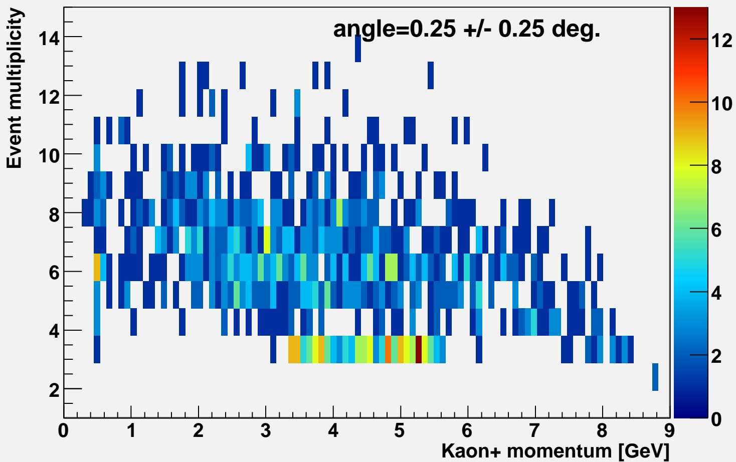
Event multiplicity vs k-momentum alpha=0.25
