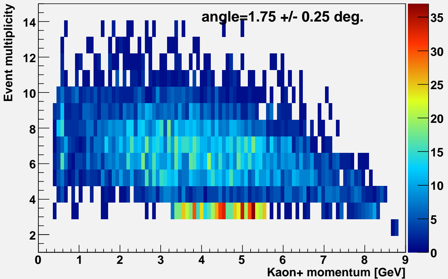
Event multiplicity vs k-momentum alpha=1.75
