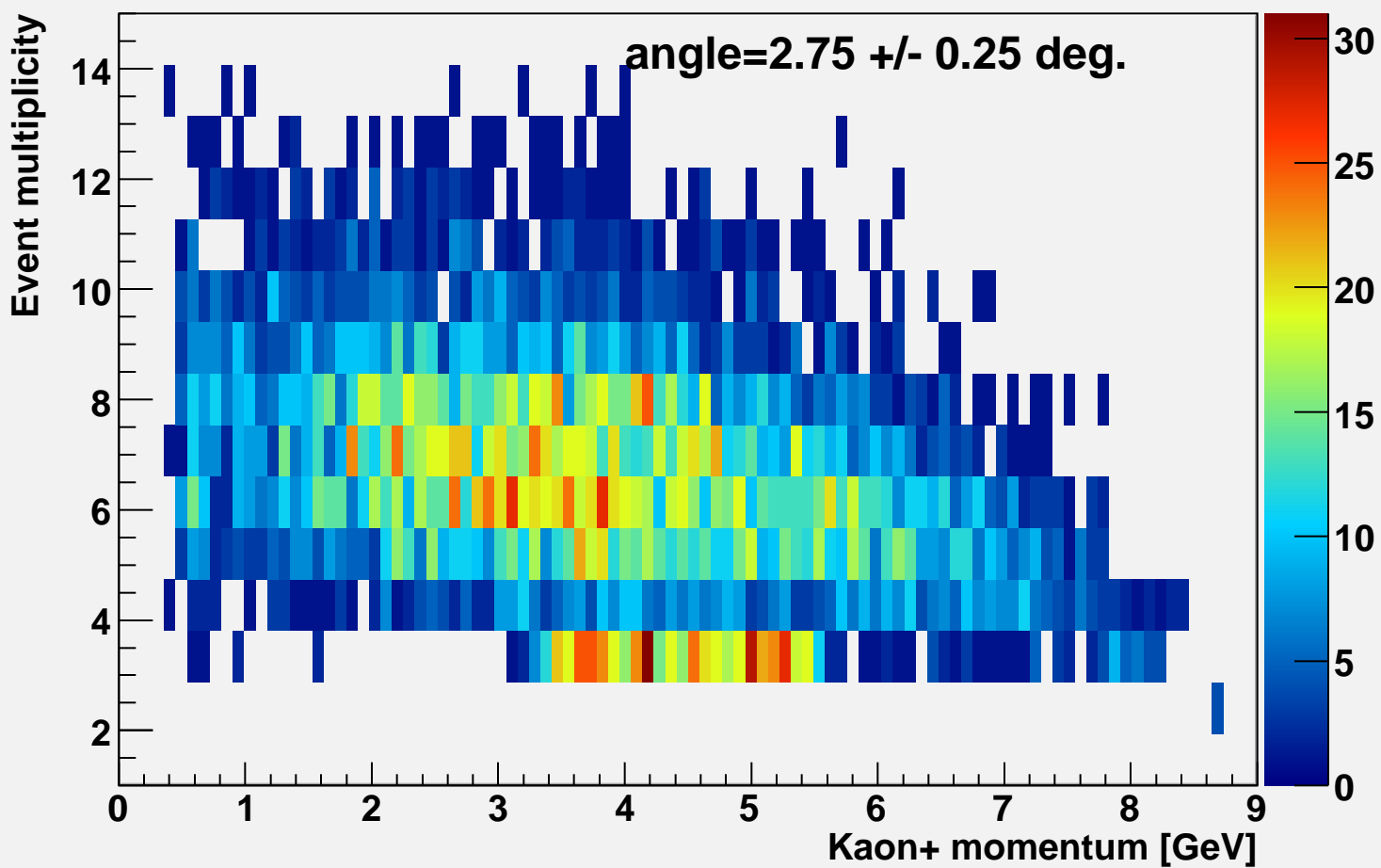
Event multiplicity vs k-momentum alpha=2.75
