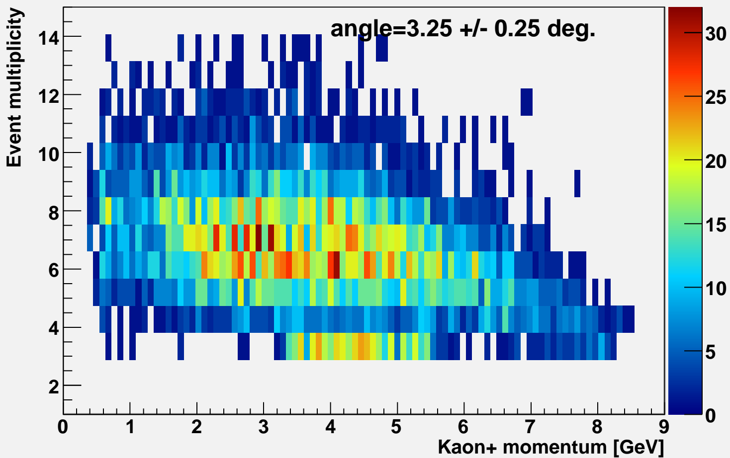
Event multiplicity vs k-momentum \alpha=3.25
