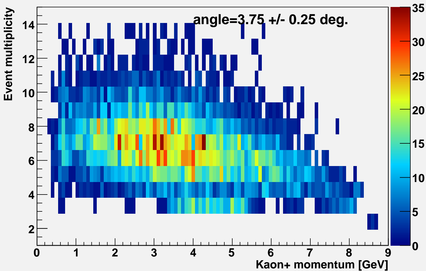
Event multiplicity vs k-momentum \alpha=3.75
