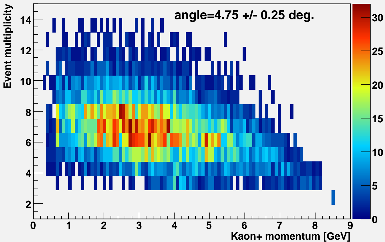
Event multiplicity vs k-momentum alpha=4.75
