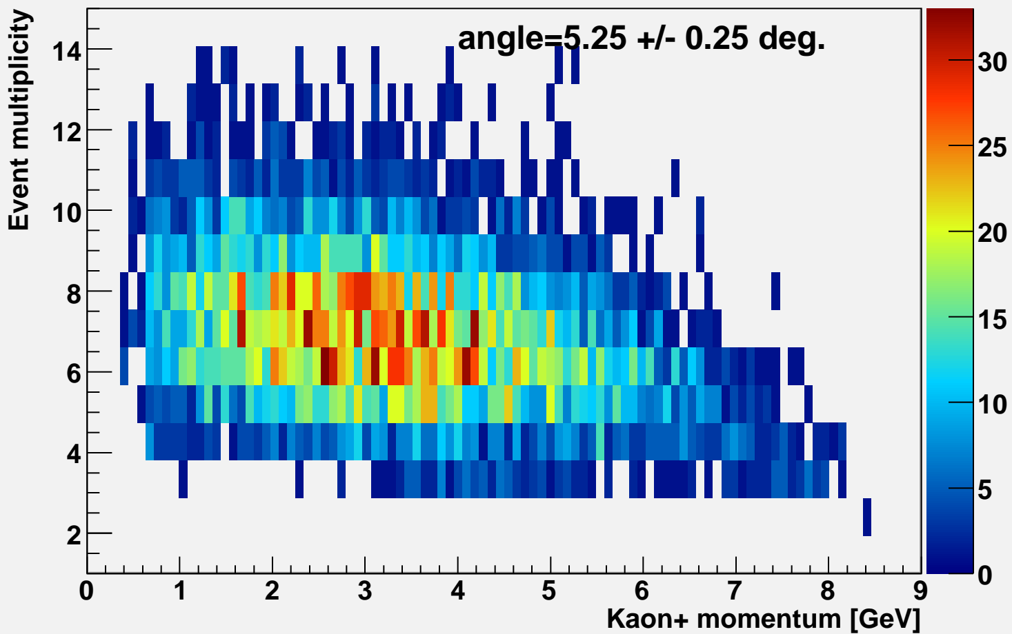
Event multiplicity vs k-momentum alpha=5.25
