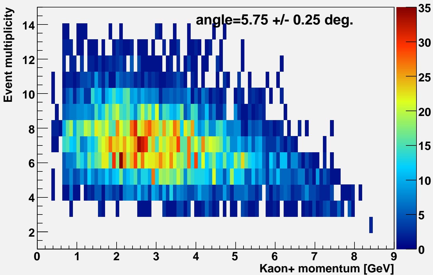
Event multiplicity vs k-momentum alpha=5.75
