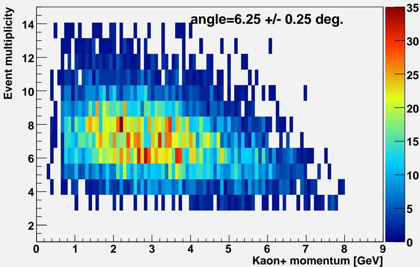
Event multiplicity vs k-momentum alpha=6.25
