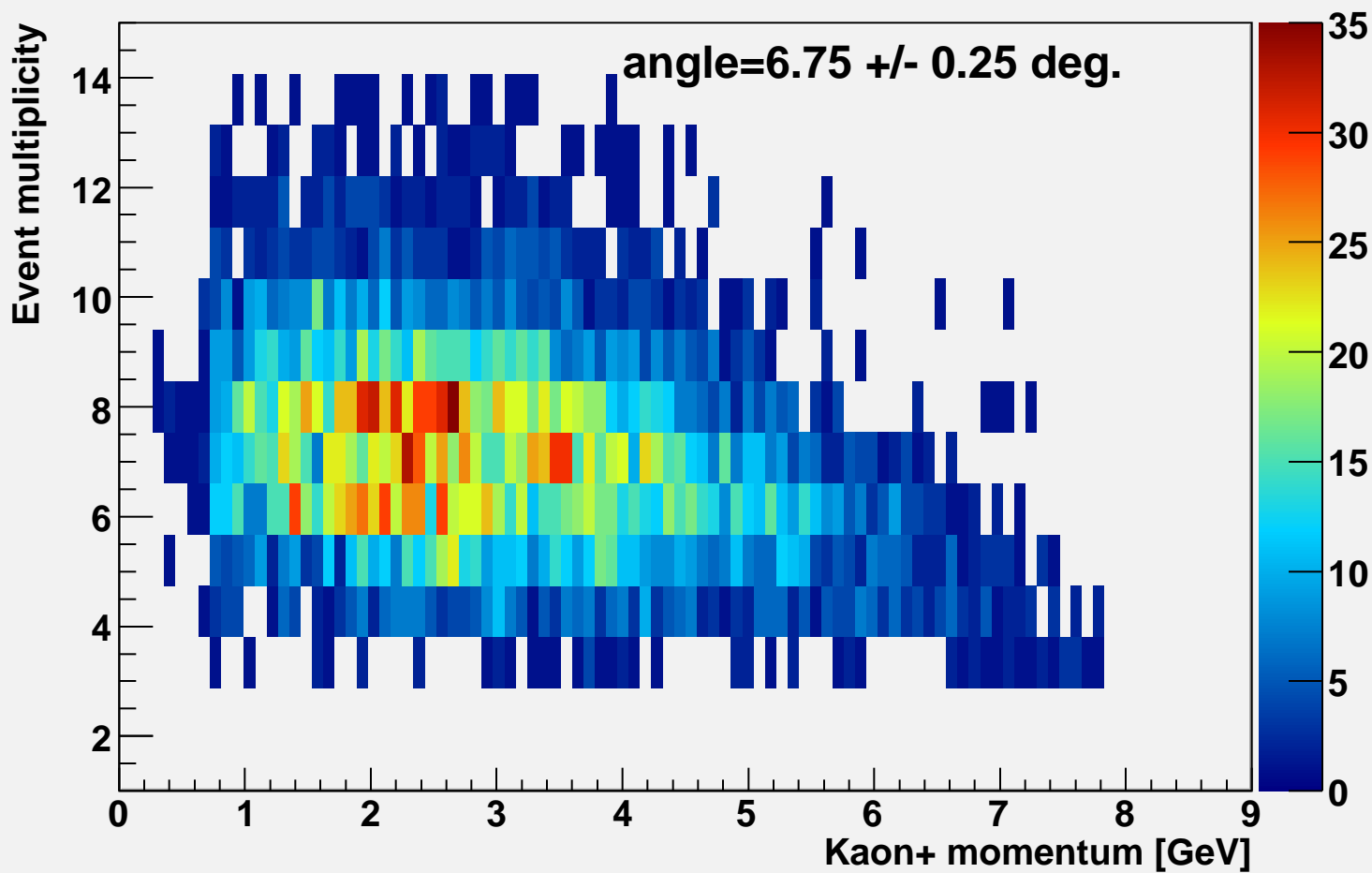
Event multiplicity vs k-momentum alpha=6.75
