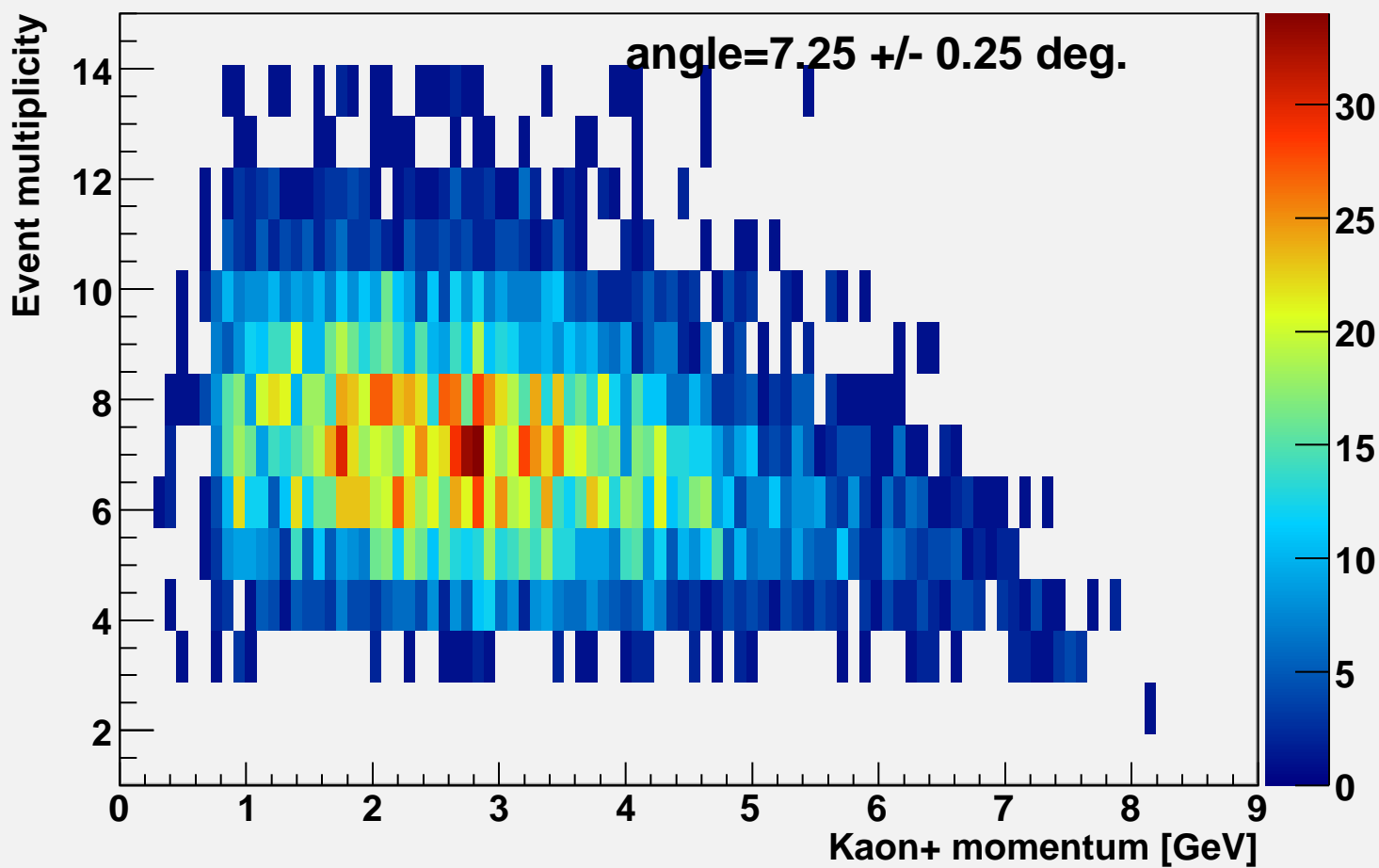
Event multiplicity vs k-momentum alpha=7.25
