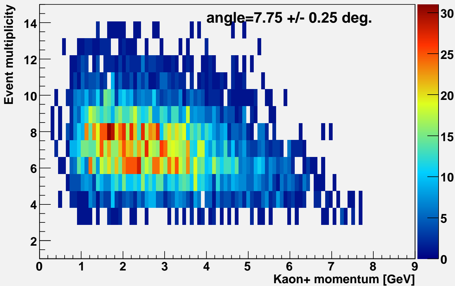
Event multiplicity vs k-momentum alpha=7.75
