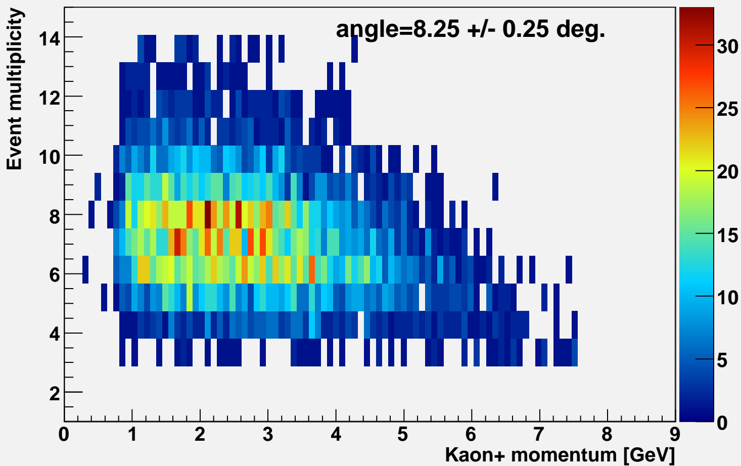
Event multiplicity vs k-momentum alpha=8.25
