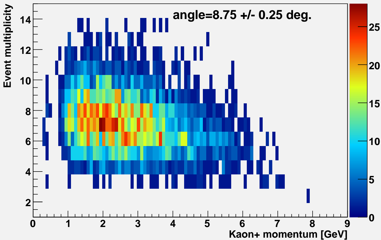
Event multiplicity vs k-momentum alpha=8.75
