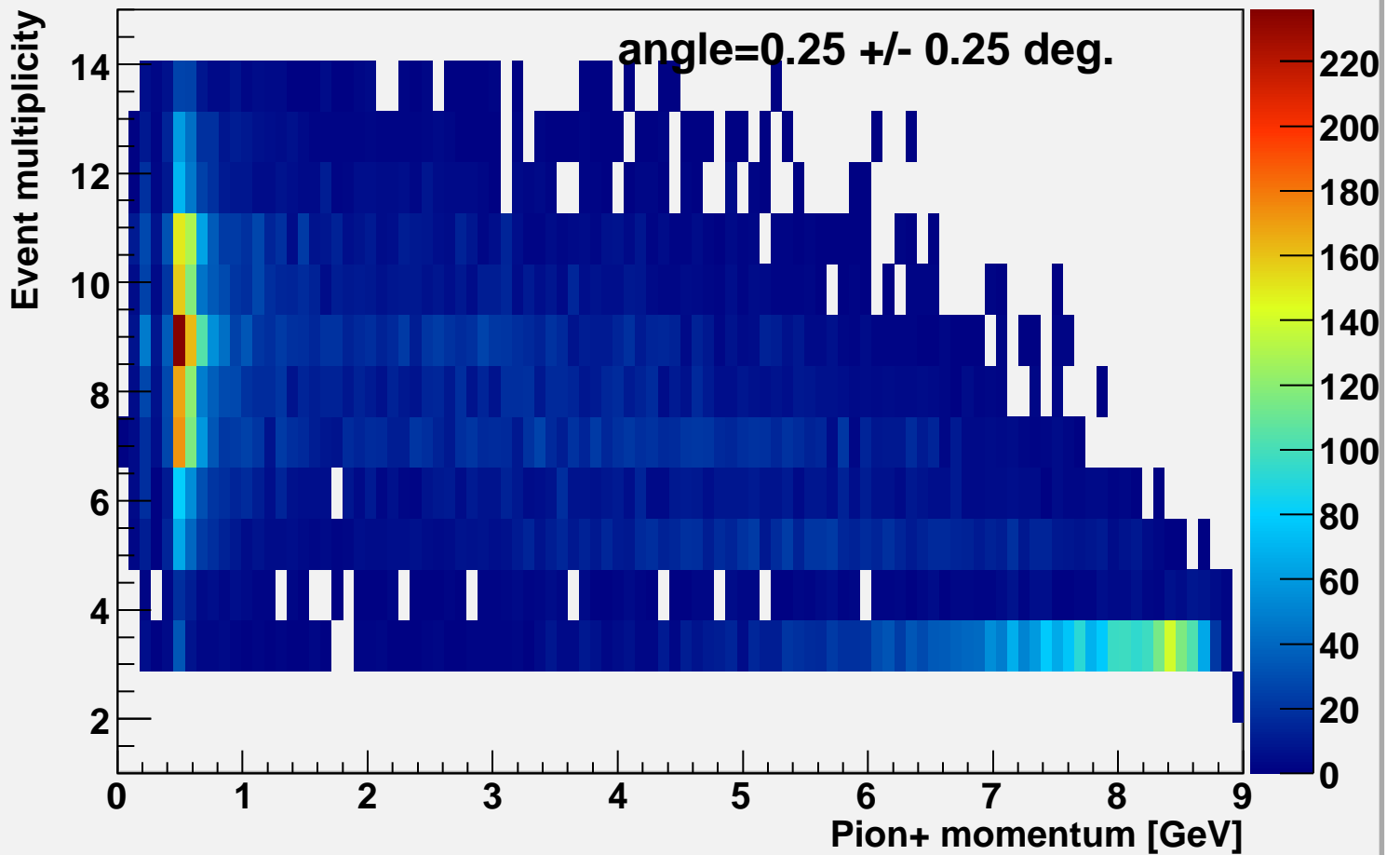
Event multiplicity vs pi-momentum alpha=0.25
