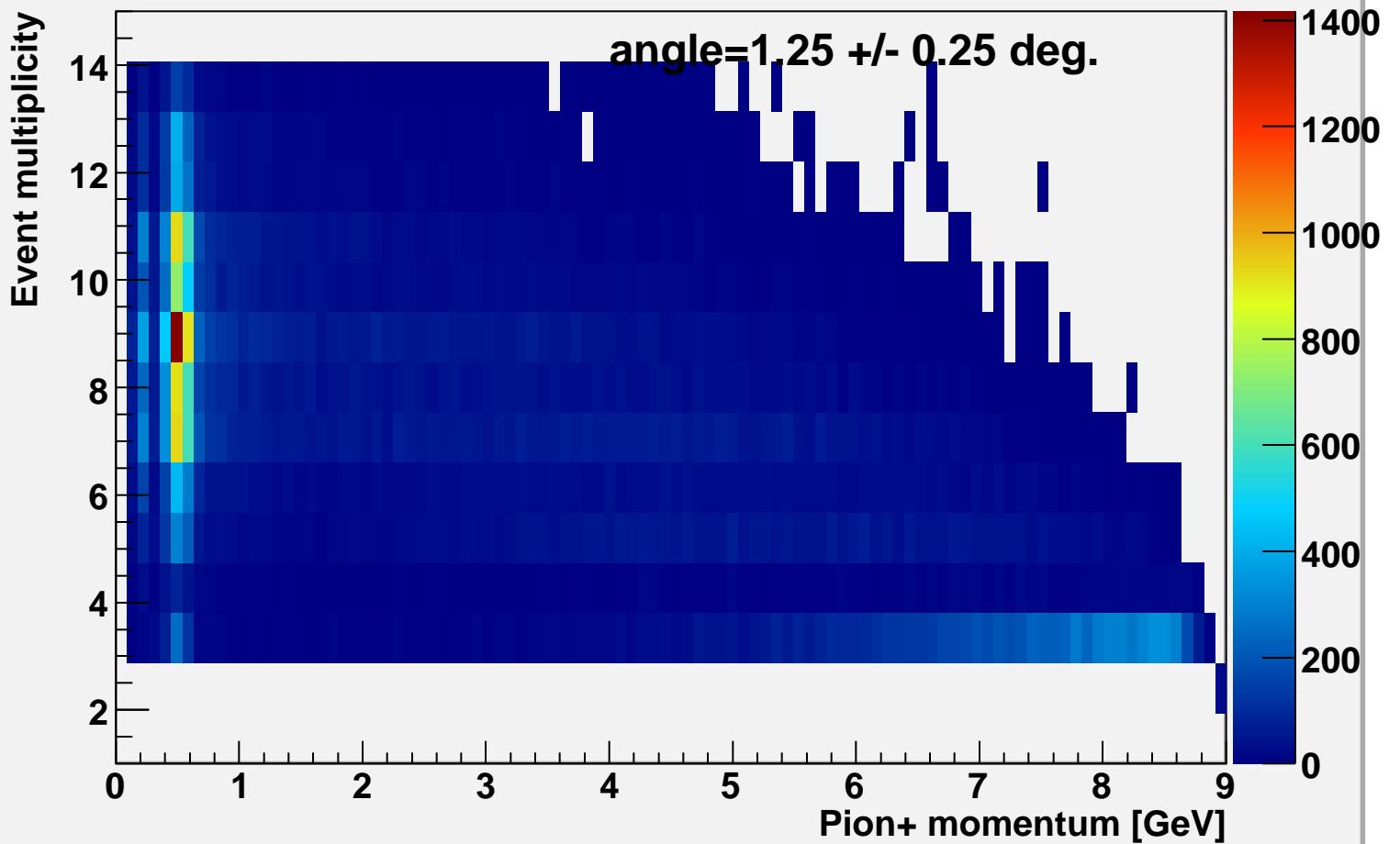
Event multiplicity vs pi-momentum alpha=1.25
