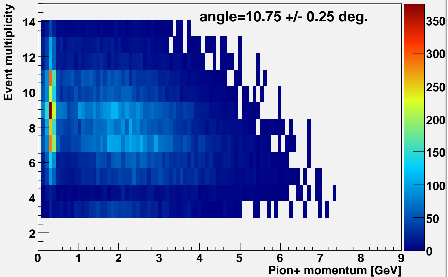
Event multiplicity vs pi-momentum alpha=10.75
