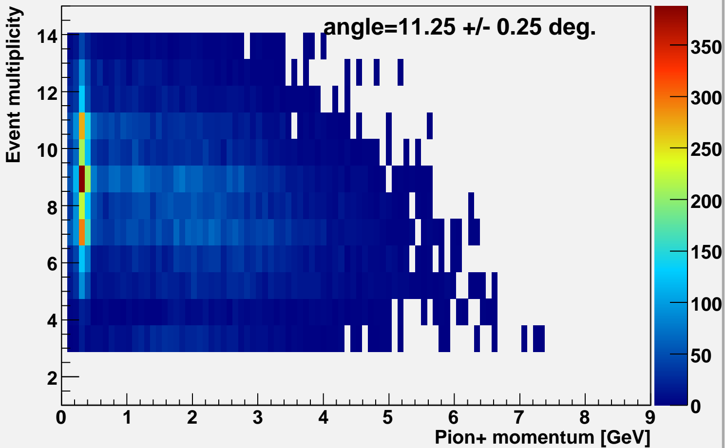
Event multiplicity vs pi-momentum alpha=11.25
