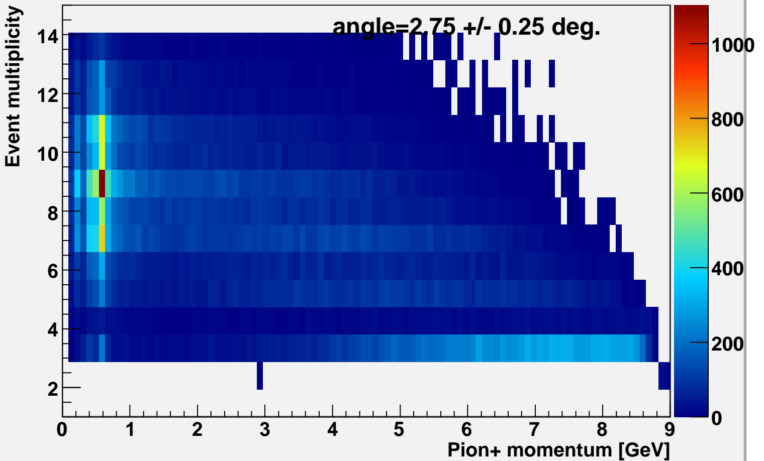
Event multiplicity vs pi-momentum alpha=2.75
