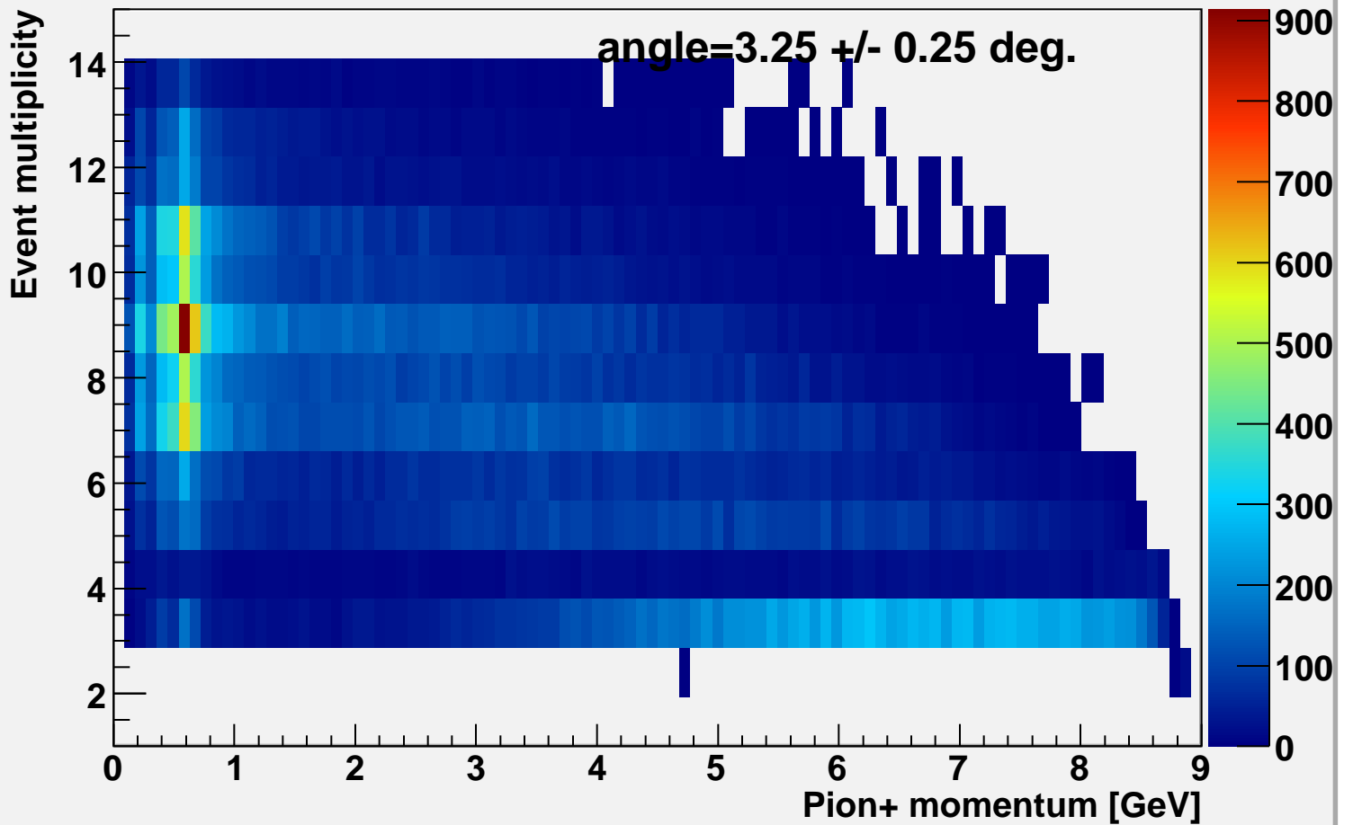
Event multiplicity vs pi-momentum alpha=3.25
