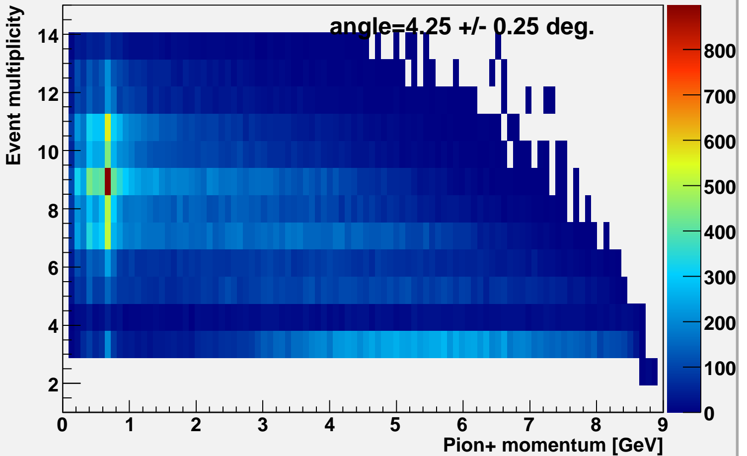
Event multiplicity vs pi-momentum alpha=4.25
