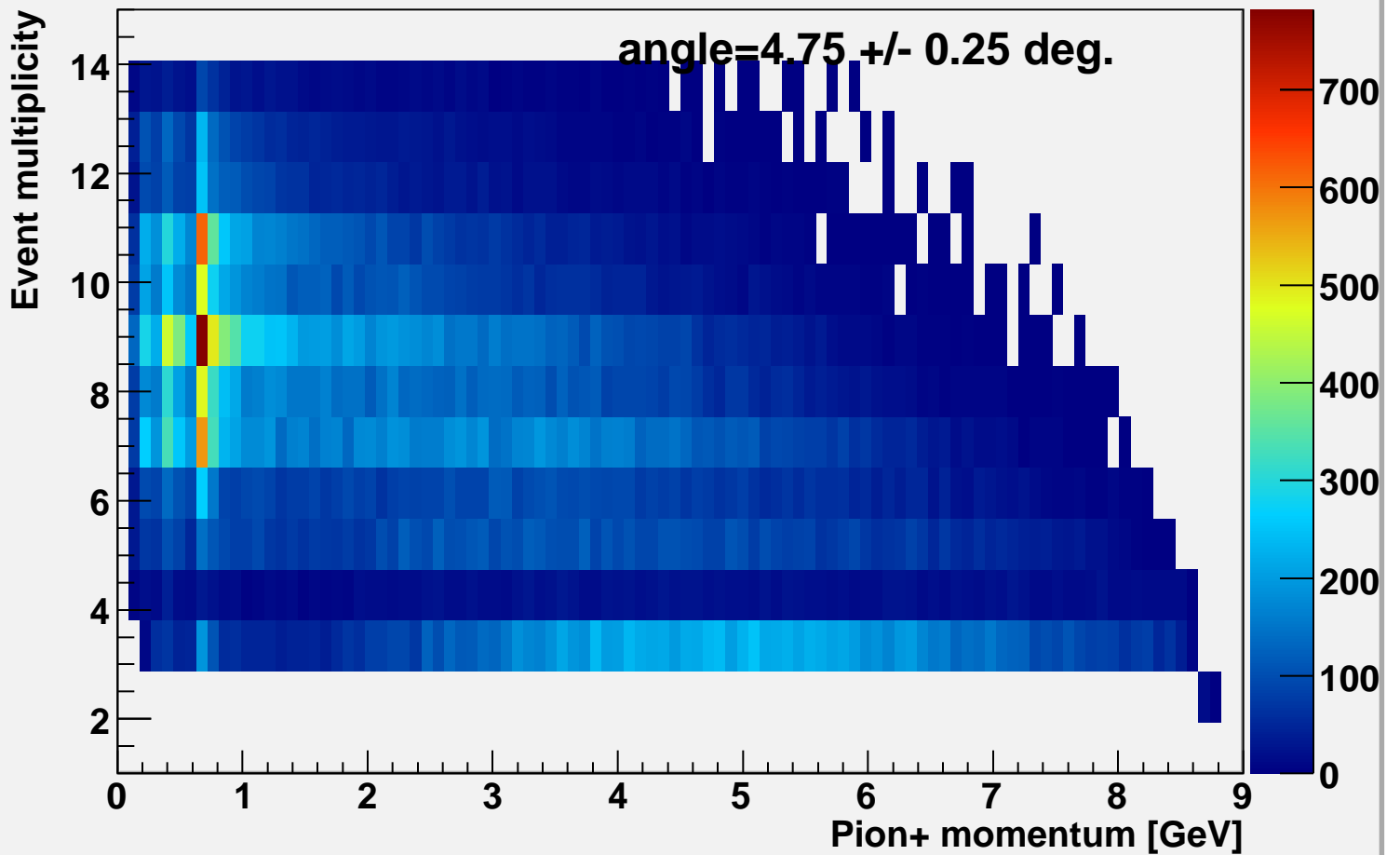
Event multiplicity vs pi-momentum alpha=4.75
