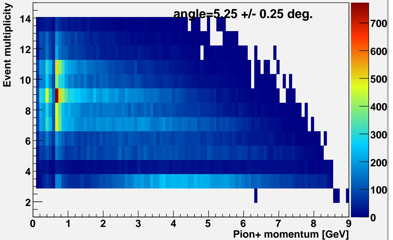
Event multiplicity vs pi-momentum alpha=5.25
