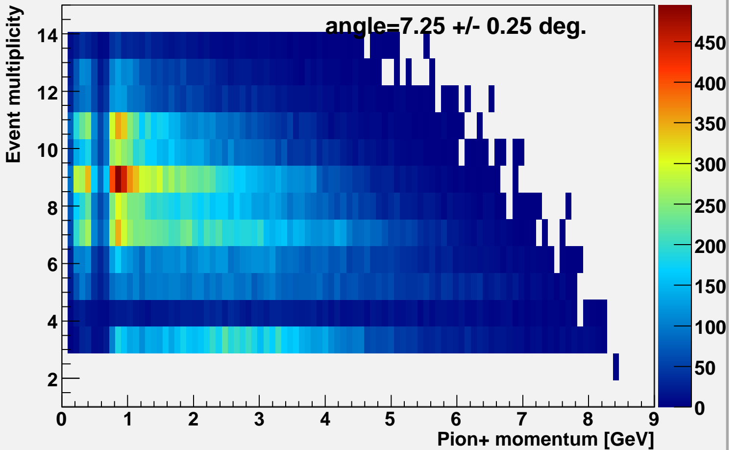
Event multiplicity vs pi-momentum alpha=7.25
