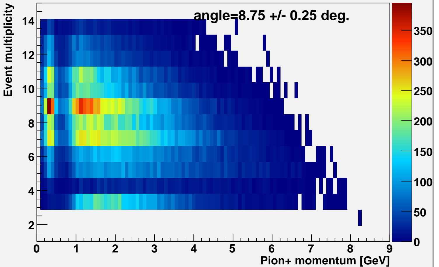
Event multiplicity vs pi-momentum alpha=8.75
