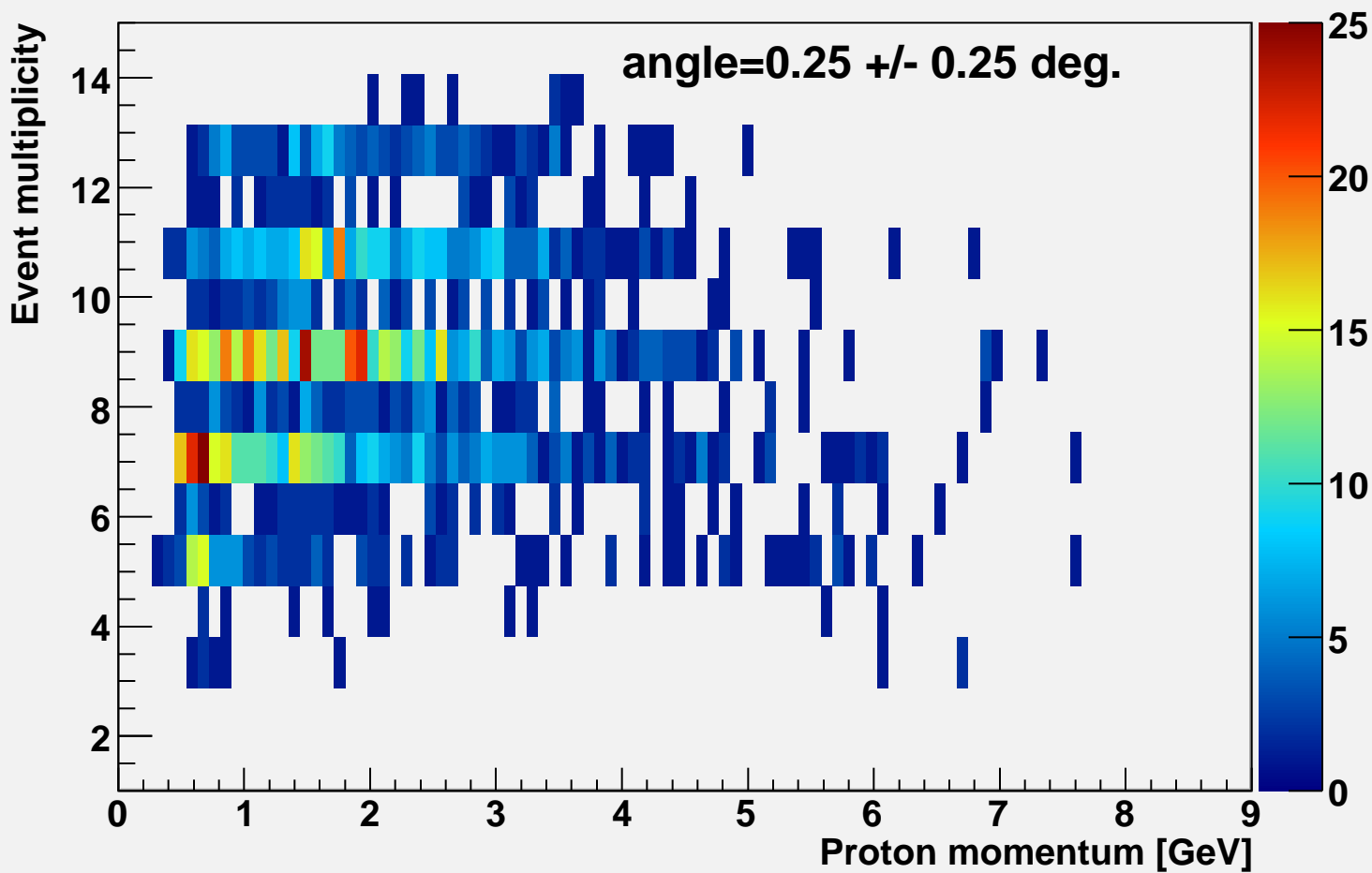
Event multiplicity vs p-momentum alpha=0.25
