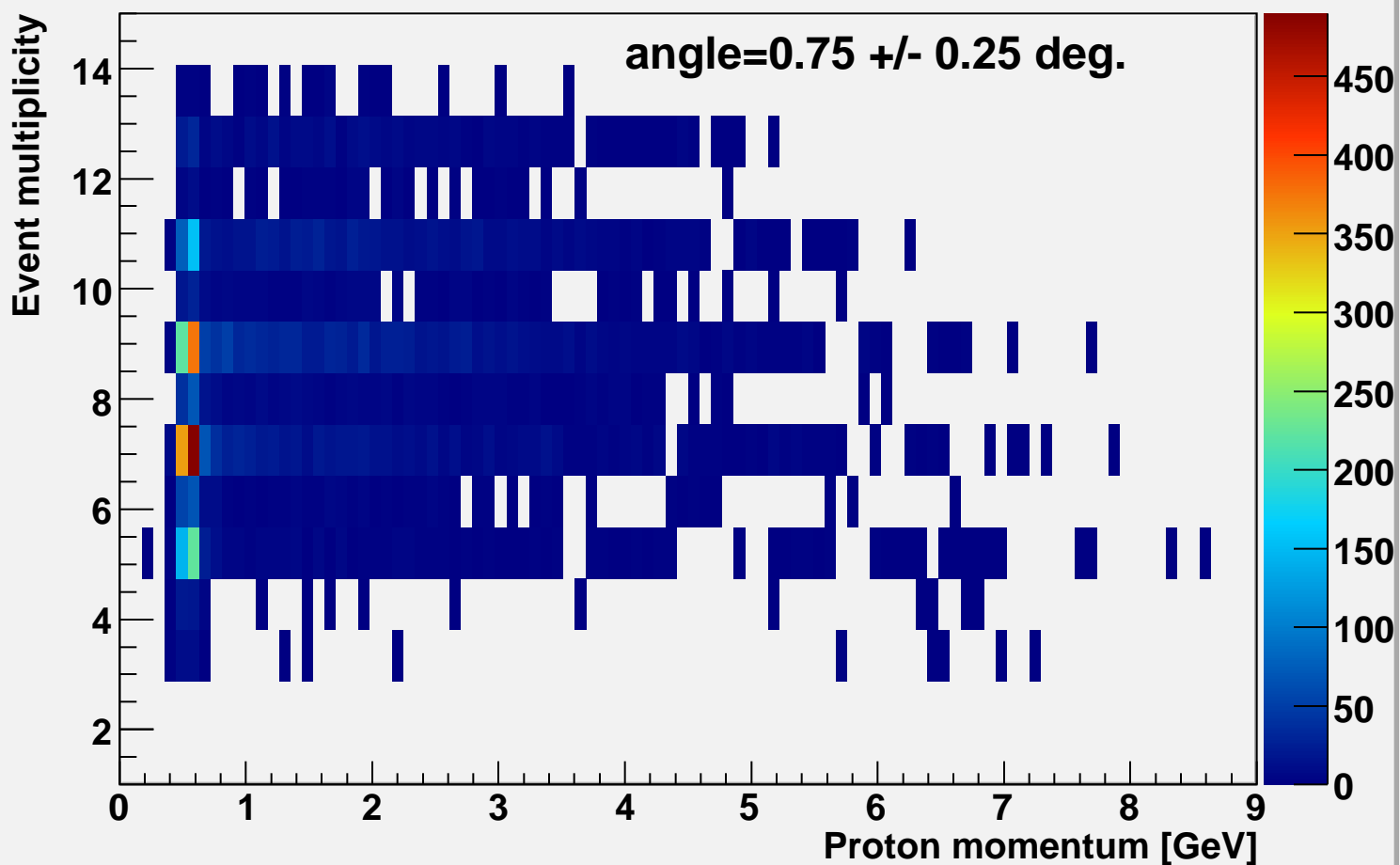
Event multiplicity vs p-momentum alpha=0.75
