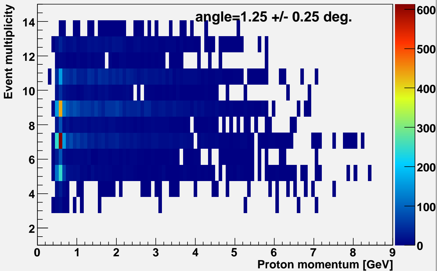
Event multiplicity vs p-momentum alpha=1.25
