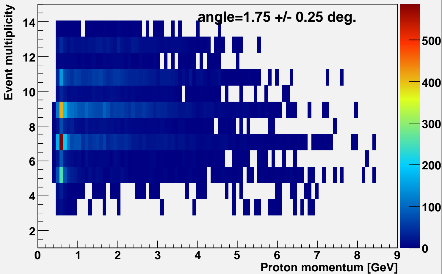
Event multiplicity vs p-momentum alpha=1.75
