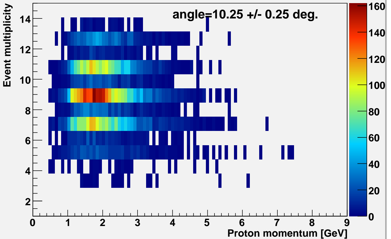
Event multiplicity vs p-momentum alpha=10.25
