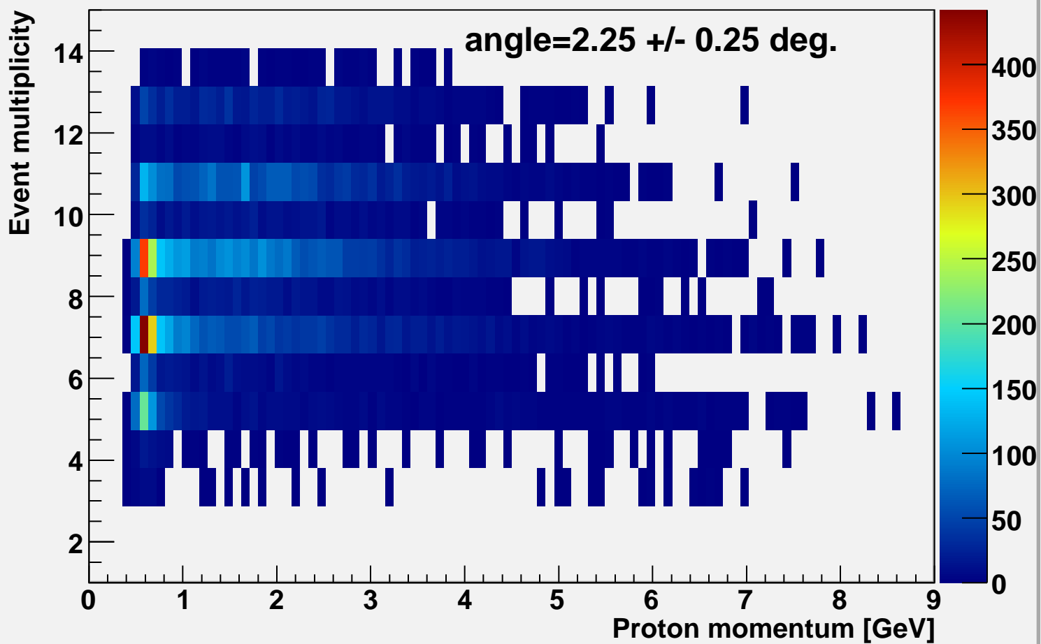
Event multiplicity vs p-momentum alpha=2.25
