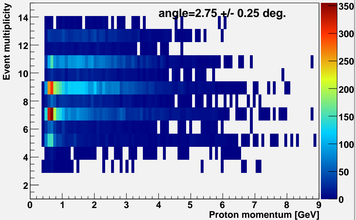
Event multiplicity vs p-momentum alpha=2.75
