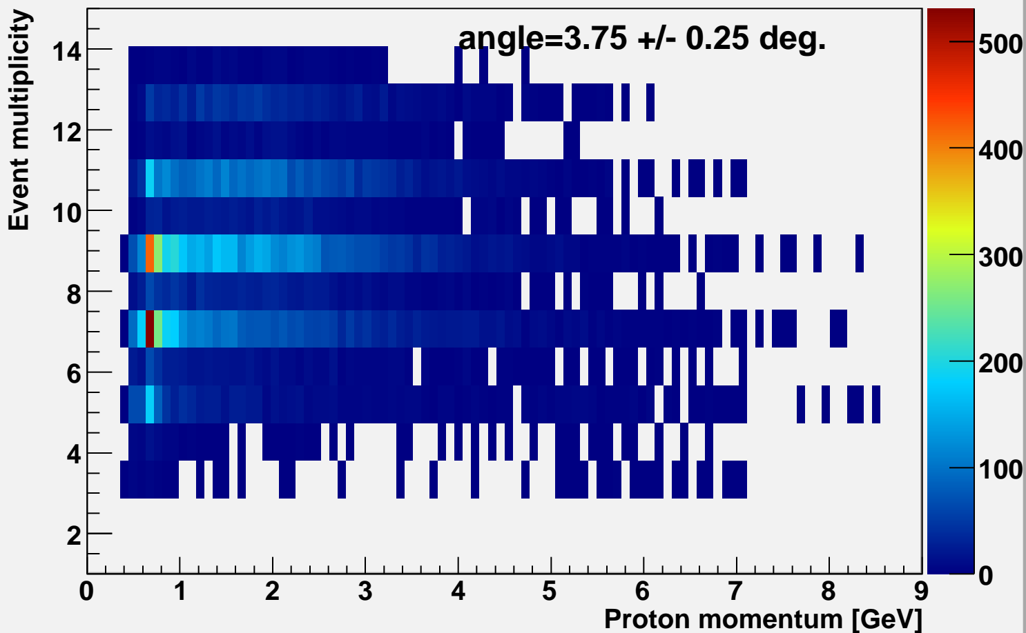
Event multiplicity vs p-momentum alpha=3.75
